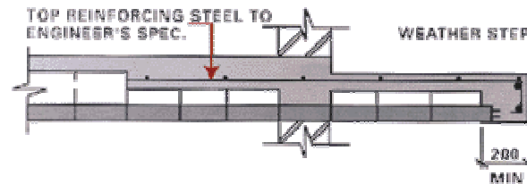
Cantilever Balcony
