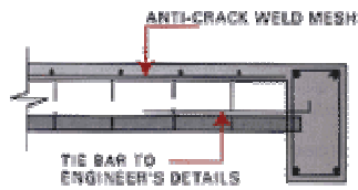
Downstand Beam
