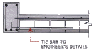
Upstand Beam
