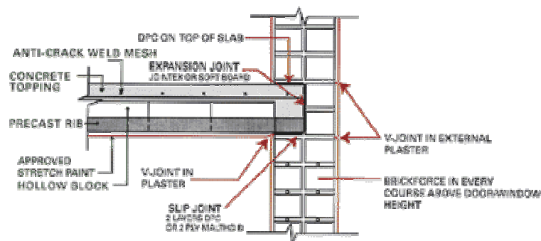
Standard Slab Detail for Load Bearing Walls
