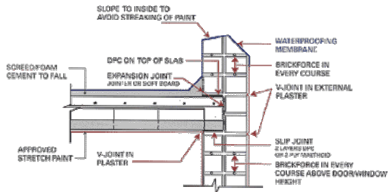
Roof Slab Parapet Wall Detail
