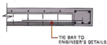
Strip Beam
